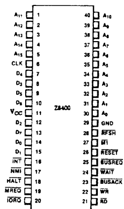
Figure 2. Pin Configuration
